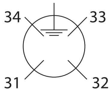
Filter 5. Connector View
