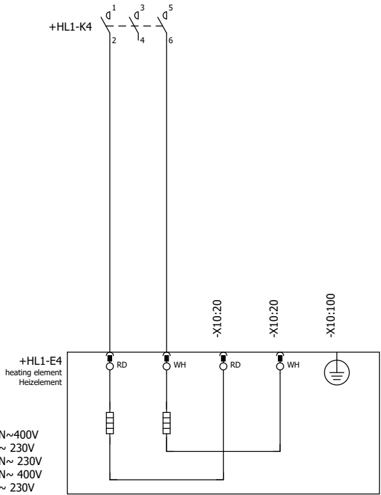
heating element 2-Phase Heizung 2-Phasen
