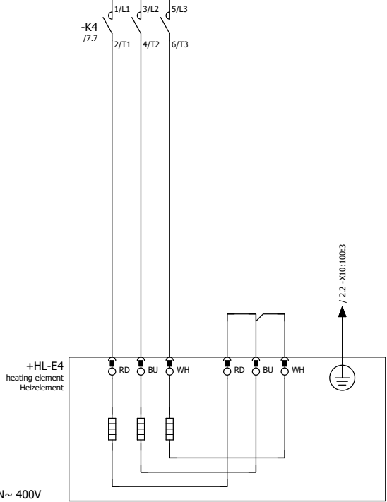
heating element 3-phase Heizung 3-Phasen
