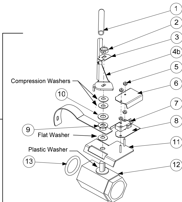
Dual-Vat Drain Valve Left Assembly 106-5607 / 106-6301 Single FP
